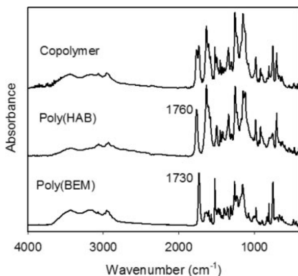
Figure 3 The FTIR spectra of poly(BEM), poly(HAB), and copolymer.
