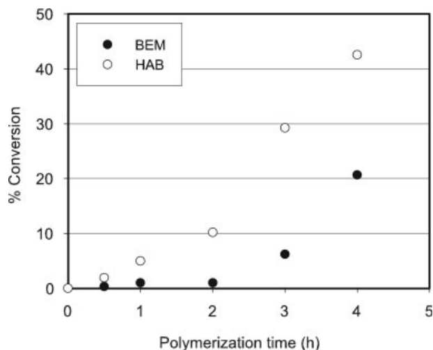
Figure 2 The % conversion of the comonomer system, 1.5 mM BEM and 1.5 mM HAB, during polymerization using 1.5 mM ammonium persulfate, 0.6 mM DBSA, and 0.15M NaCl at 70°C.
