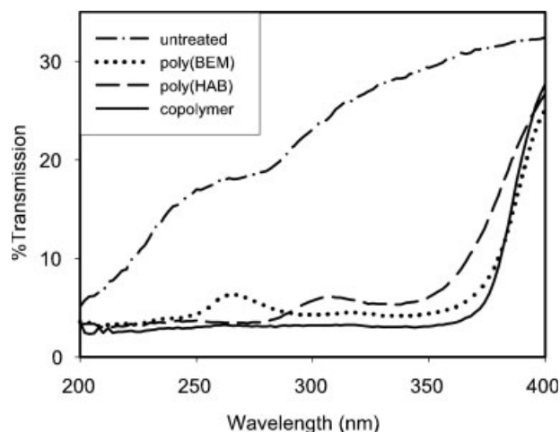
Figure 9 The % UV transmission of untreated cotton fabric, cotton fabrics coated by homopolymers using 0.8 mM BEM, and 0.8 mM HAB, and cotton fabric coated by copolymer using 0.4 mM BEM and 0.4 mM HAB.
