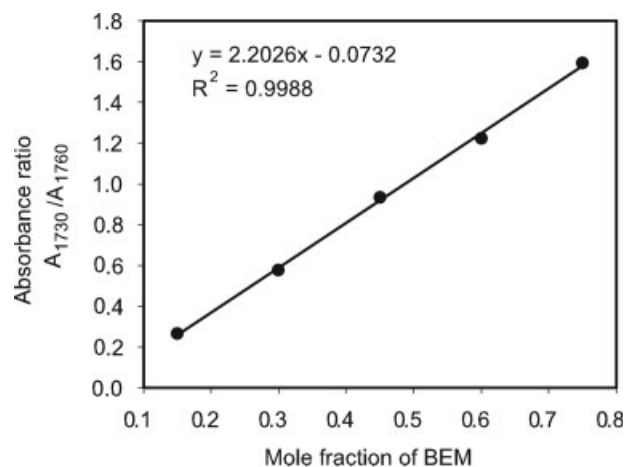
Figure 4 Calibration curve for FTIR determination of BEM content in BEM-HAB copolymer.
