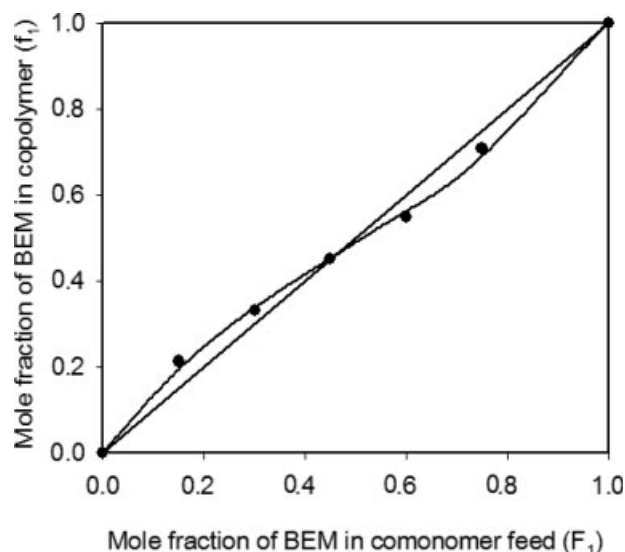
Figure 6 Comparison of the mole fraction of BEM in comonomer feed and the mole fraction of BEM in copolymer using BEM and HAB with a combined total concentration of 3.0 mM.
