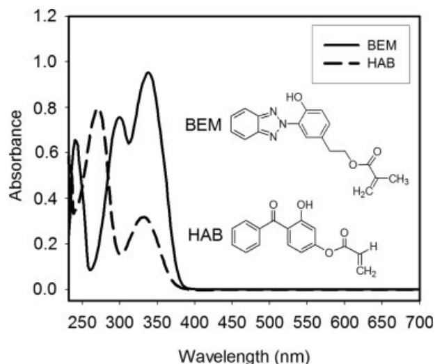
Figure 8 UV spectra of 0.05 mM BEM and 0.07 mM HAB in dichloromethane.
