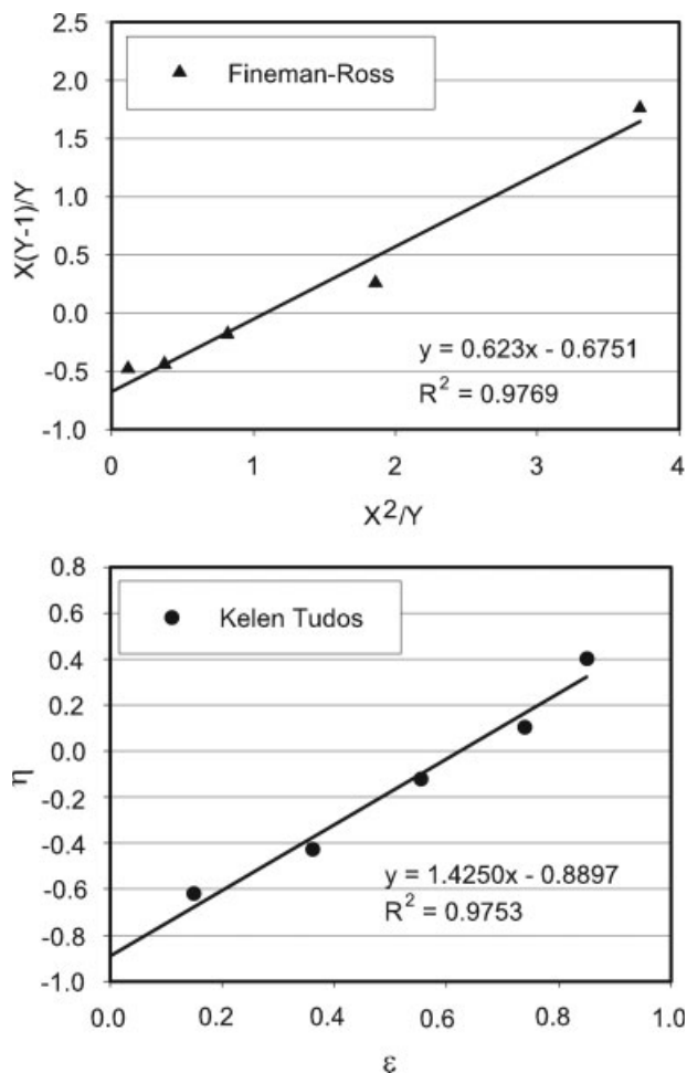
Figure 5 Fineman–Ross plot and Kelen–Tüdös plot for copolymer of BEM and HAB using BEM and HAB with a combined total concentration of 3.0 mM and mole fraction of BEM in comonomer feed varied from 0.15 to 0.75.
