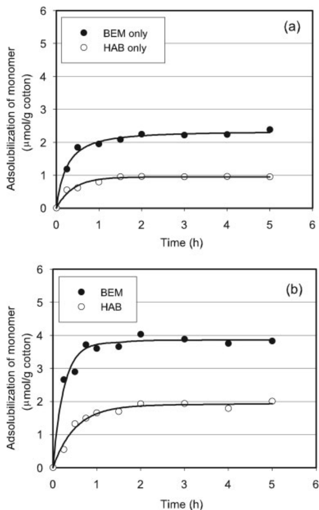
Figure 1 Adsolubilization of BEM and HAB (a) in the single system, 0.25 mM BEM/0.25 mM HAB, and (b) in the comonomer system, 0.25 mM BEM and 0.25 mM HAB, using 0.6 mM DBSA and 0.15M NaCl at 70°C.
