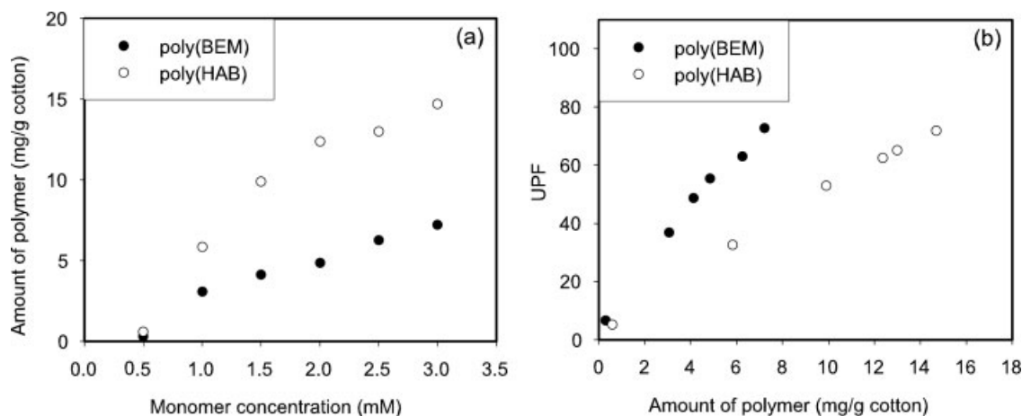
Figure 7 Relationship between (a) the amount of polymer and monomer concentration, and (b) UPF and the amount of polymer for poly(BEM) and poly(HAB).
